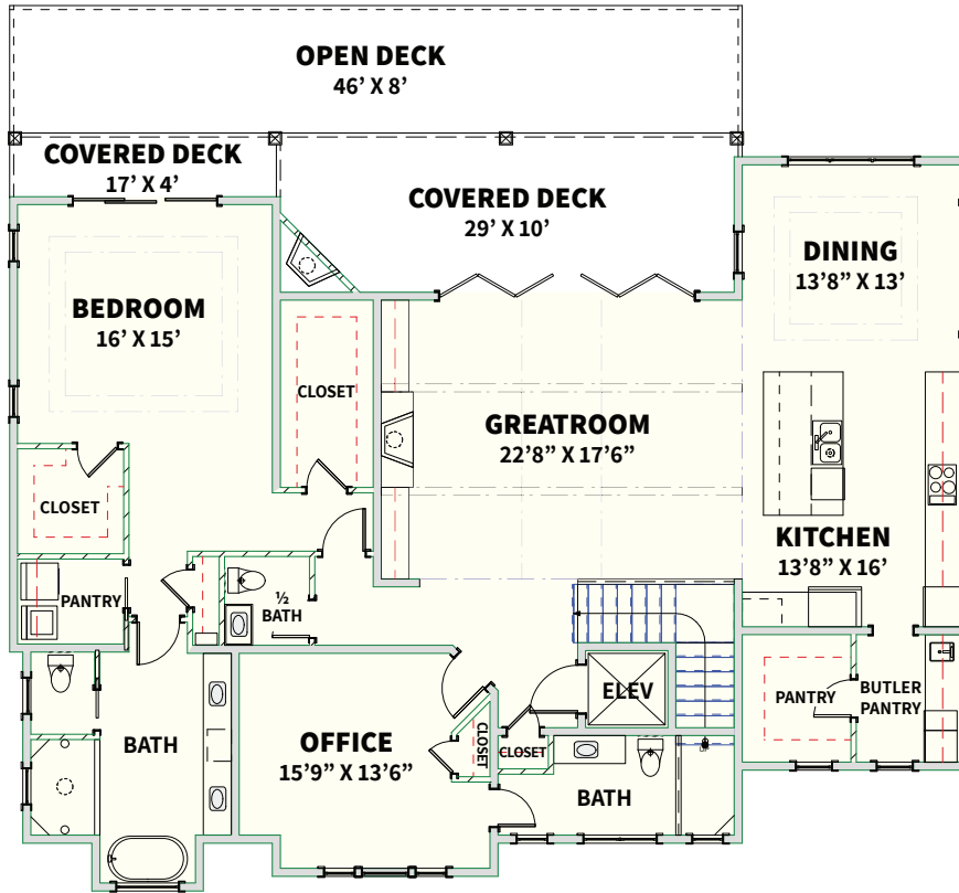
SECOND FLOOR
