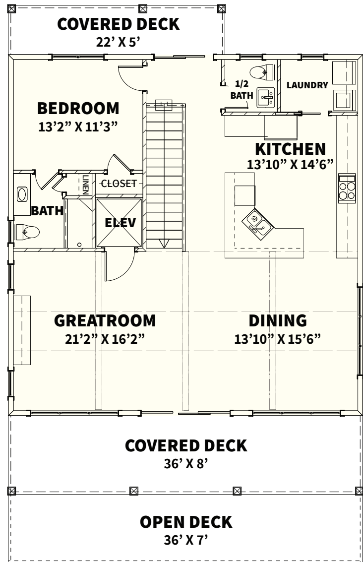
SECOND FLOOR
