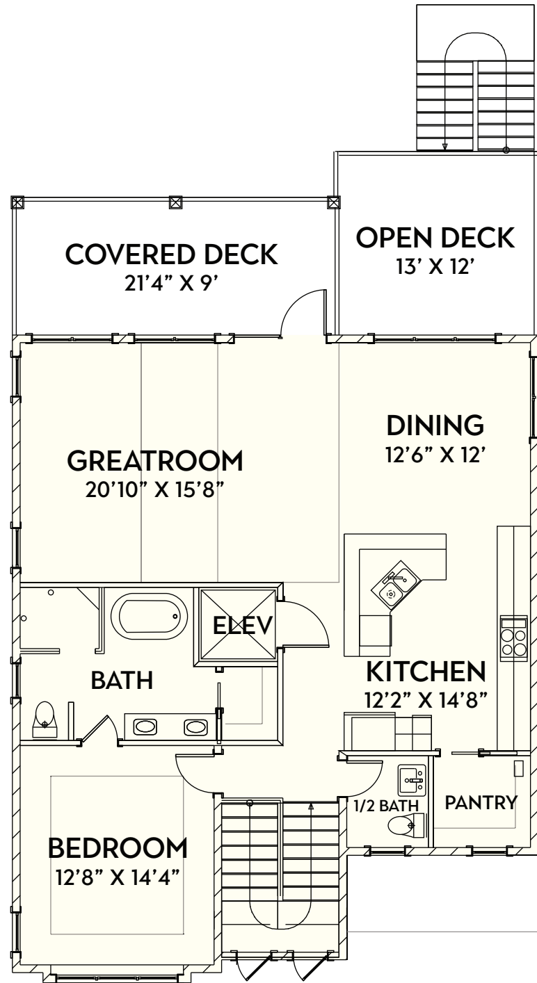
SECOND FLOOR
